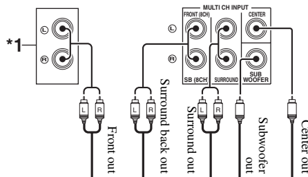
Multi-format player/External decoder (7.1-channel output)
